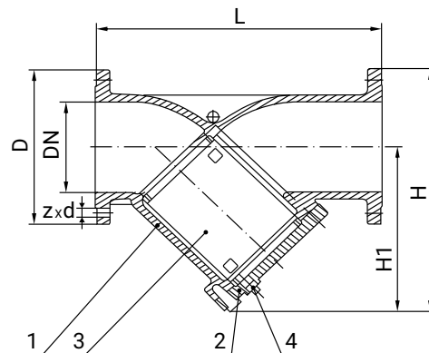
DN 50-400
