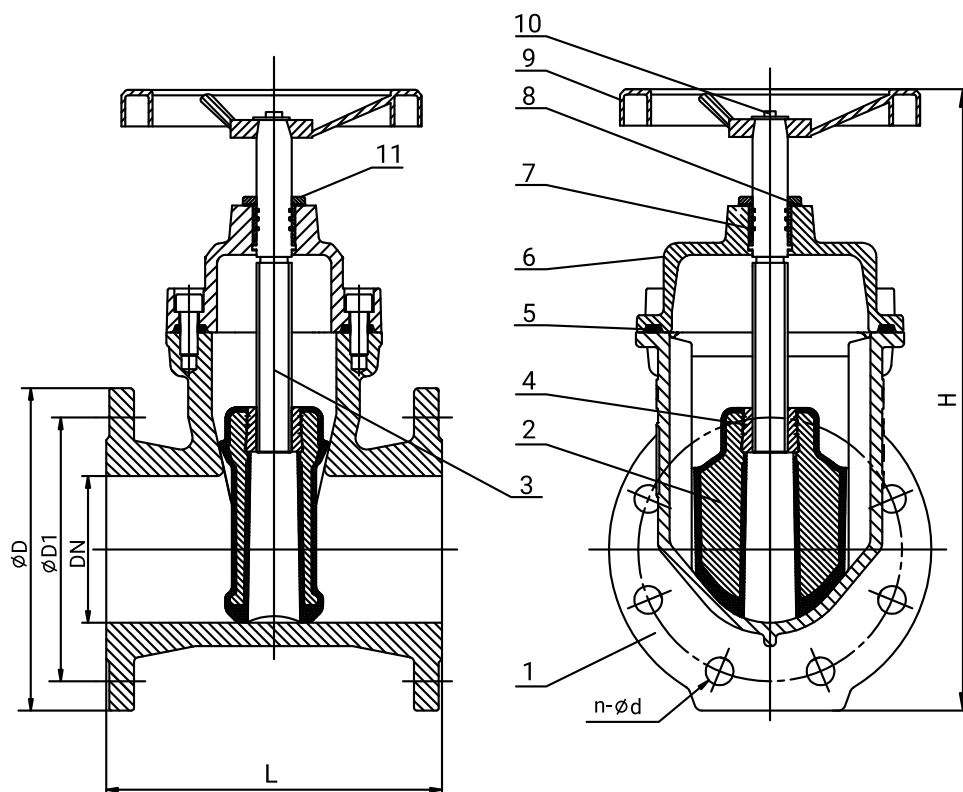
DN40-300
