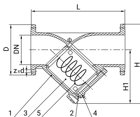
DN 50-400
